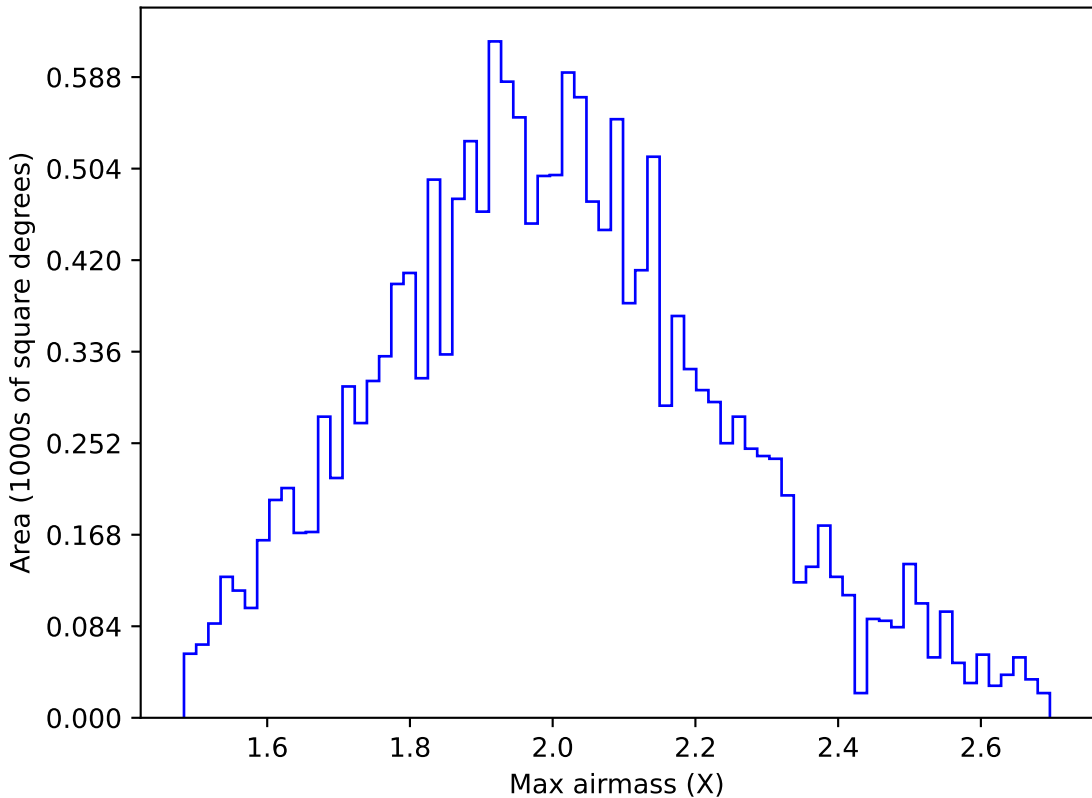
ddf_acor_sf10_lsf20_lsr20_v3.4_10yrs WFD g band: Max airmass
