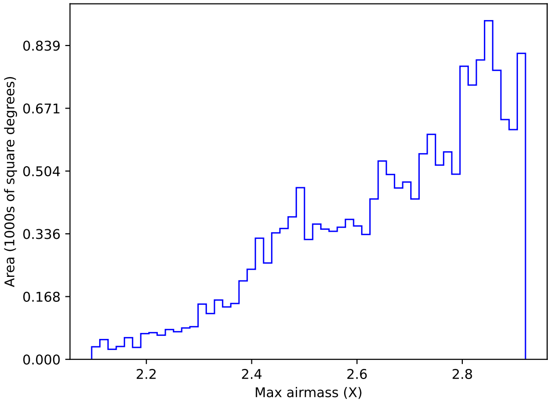
ddf_acor_sf10_lsf20_lsr20_v3.4_10yrs WFD all bands: Max airmass
