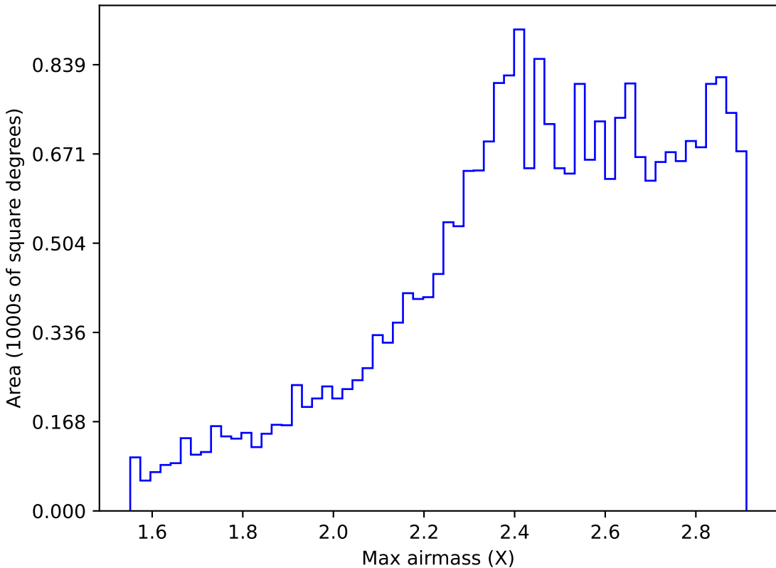
ddf_acor_sf10_lsf20_lsr20_v3.4_10yrs All sky z band: Max airmass
