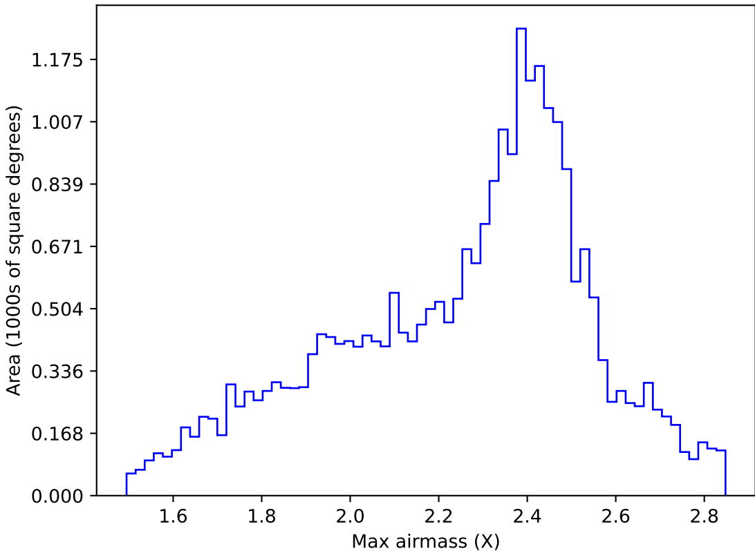
ddf_acor_sf10_lsf20_lsr20_v3.4_10yrs All sky r band: Max airmass
