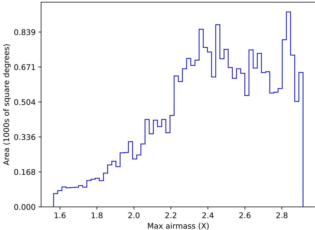
ddf_acor_sf10_lsf20_lsr20_v3.4_10yrs All sky i band: Max airmass
