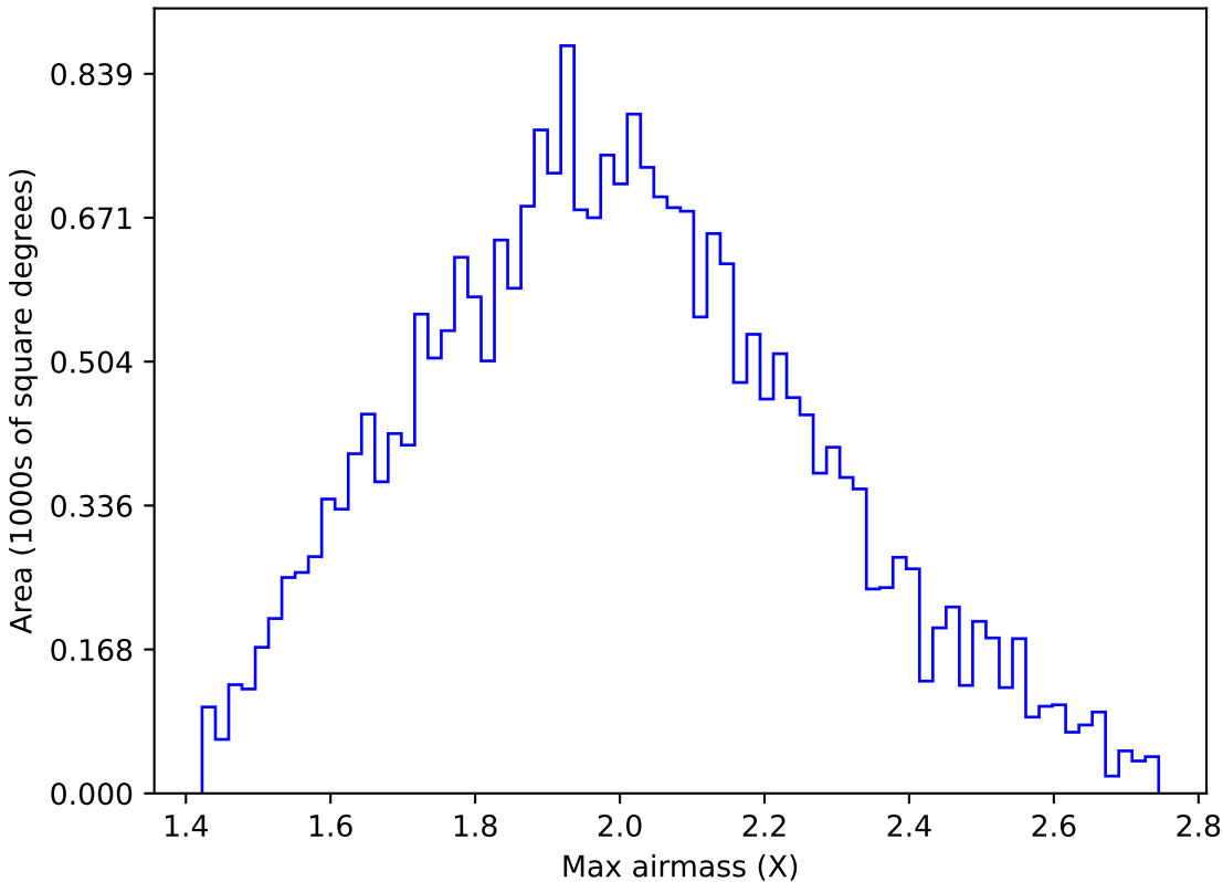
ddf_acor_sf10_lsf20_lsr20_v3.4_10yrs All sky g band: Max airmass
