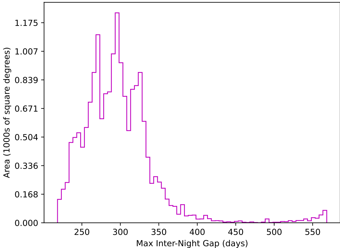
ddf_acor_sf10_lsf20_lsr20_v3.4_10yrs WFD z band: Max Inter-Night Gap
