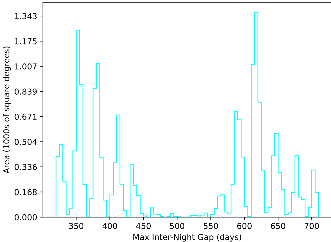
ddf_acor_sf10_lsf20_lsr20_v3.4_10yrs WFD u band: Max Inter-Night Gap
