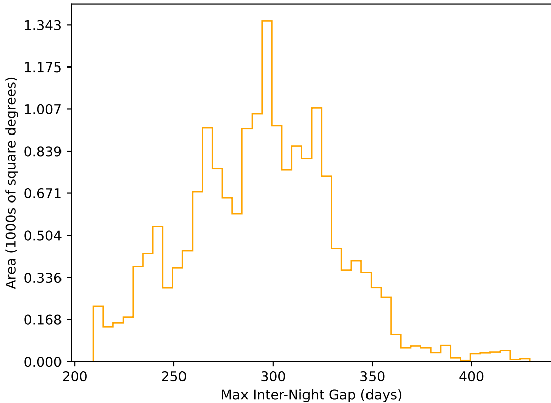
ddf_acor_sf10_lsf20_lsr20_v3.4_10yrs WFD r band: Max Inter-Night Gap
