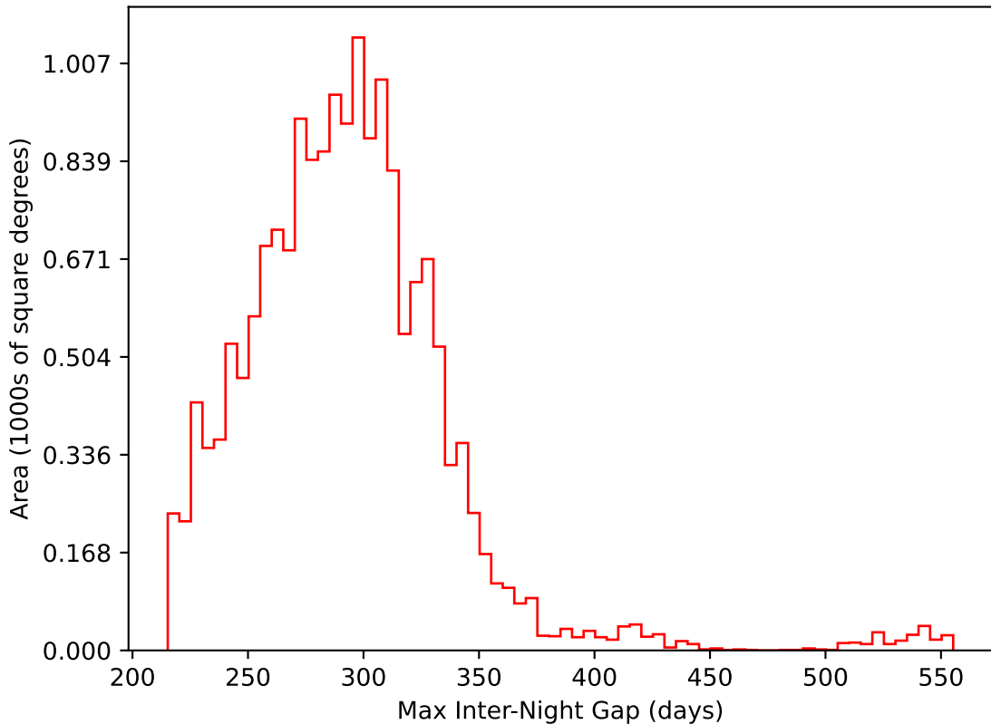
ddf_acor_sf10_lsf20_lsr20_v3.4_10yrs WFD i band: Max Inter-Night Gap
