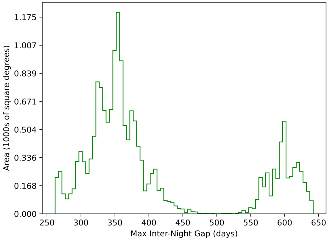
ddf_acor_sf10_lsf20_lsr20_v3.4_10yrs WFD g band: Max Inter-Night Gap
