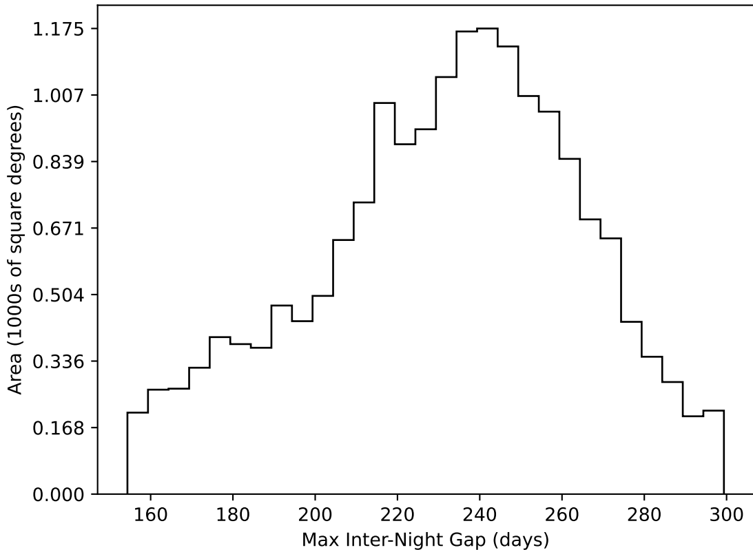
ddf_acor_sf10_lsf20_lsr20_v3.4_10yrs WFD all bands: Max Inter-Night Gap
