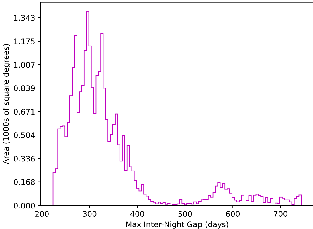
ddf_acor_sf10_lsf20_lsr20_v3.4_10yrs All sky z band: Max Inter-Night Gap
