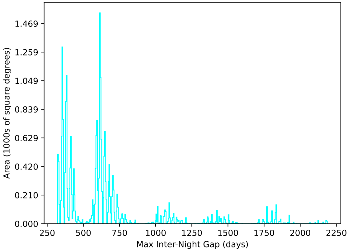
ddf_acor_sf10_lsf20_lsr20_v3.4_10yrs All sky u band: Max Inter-Night Gap
