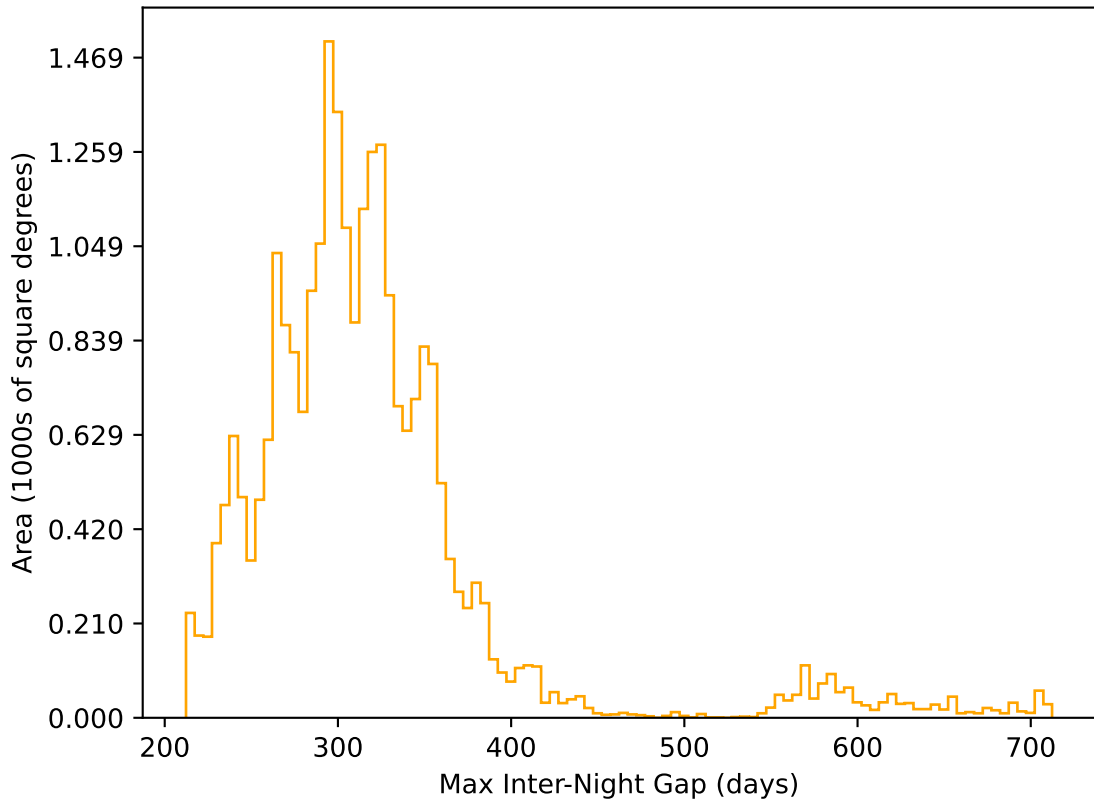
ddf_acor_sf10_lsf20_lsr20_v3.4_10yrs All sky r band: Max Inter-Night Gap
