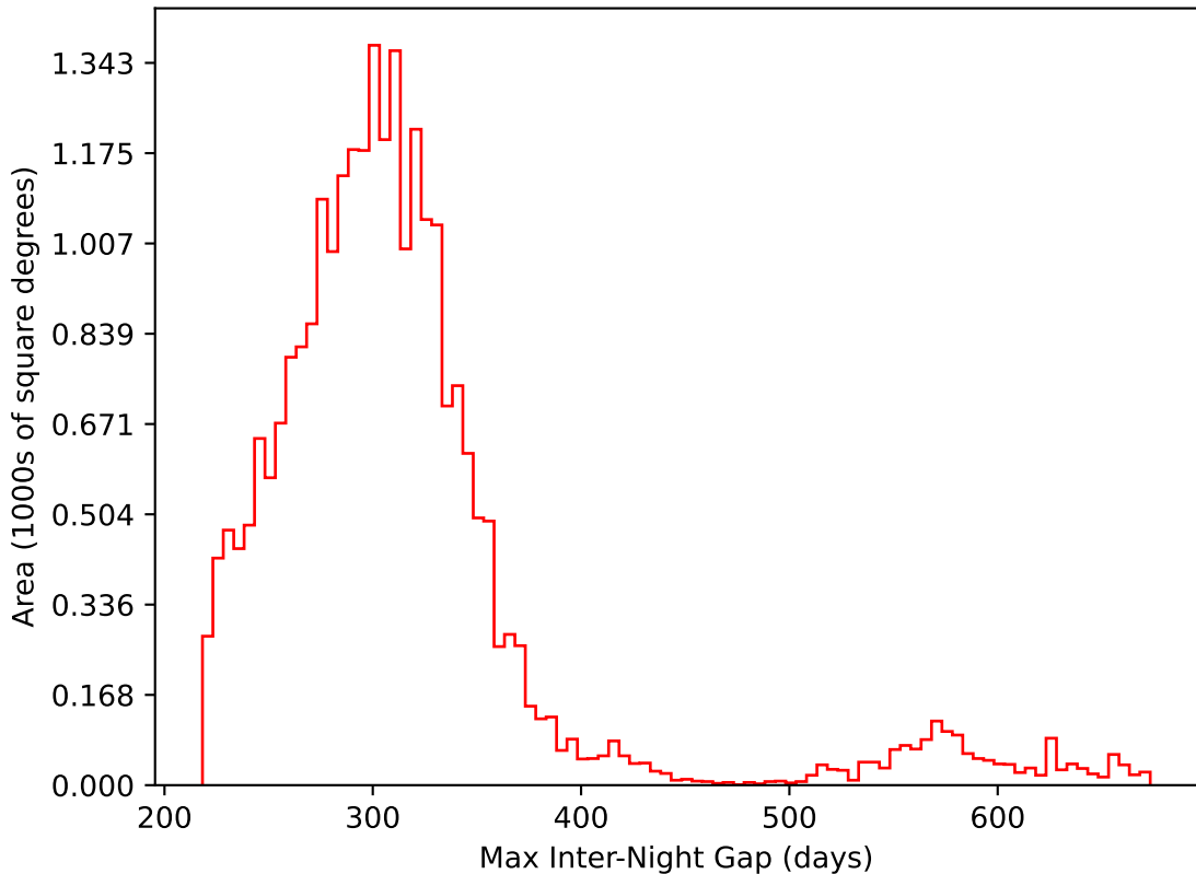
ddf_acor_sf10_lsf20_lsr20_v3.4_10yrs All sky i band: Max Inter-Night Gap
