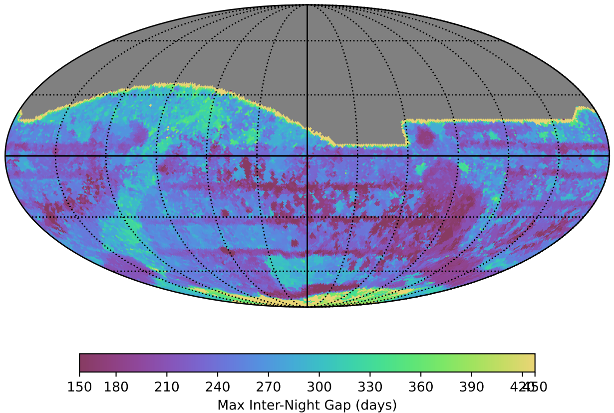
ddf_acor_sf10_lsf20_lsr20_v3.4_10yrs All sky all bands: Max Inter-Night Gap
