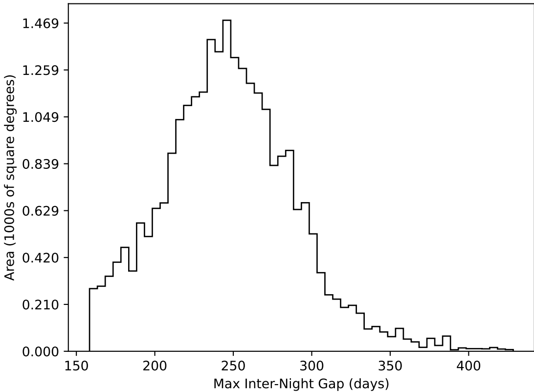
ddf_acor_sf10_lsf20_lsr20_v3.4_10yrs All sky all bands: Max Inter-Night Gap
