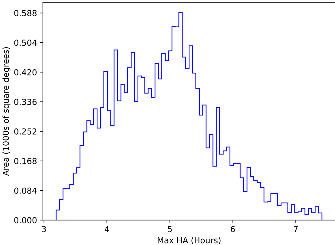
ddf_acor_sf10_lsf20_lsr20_v3.4_10yrs WFD z band: Max HA
