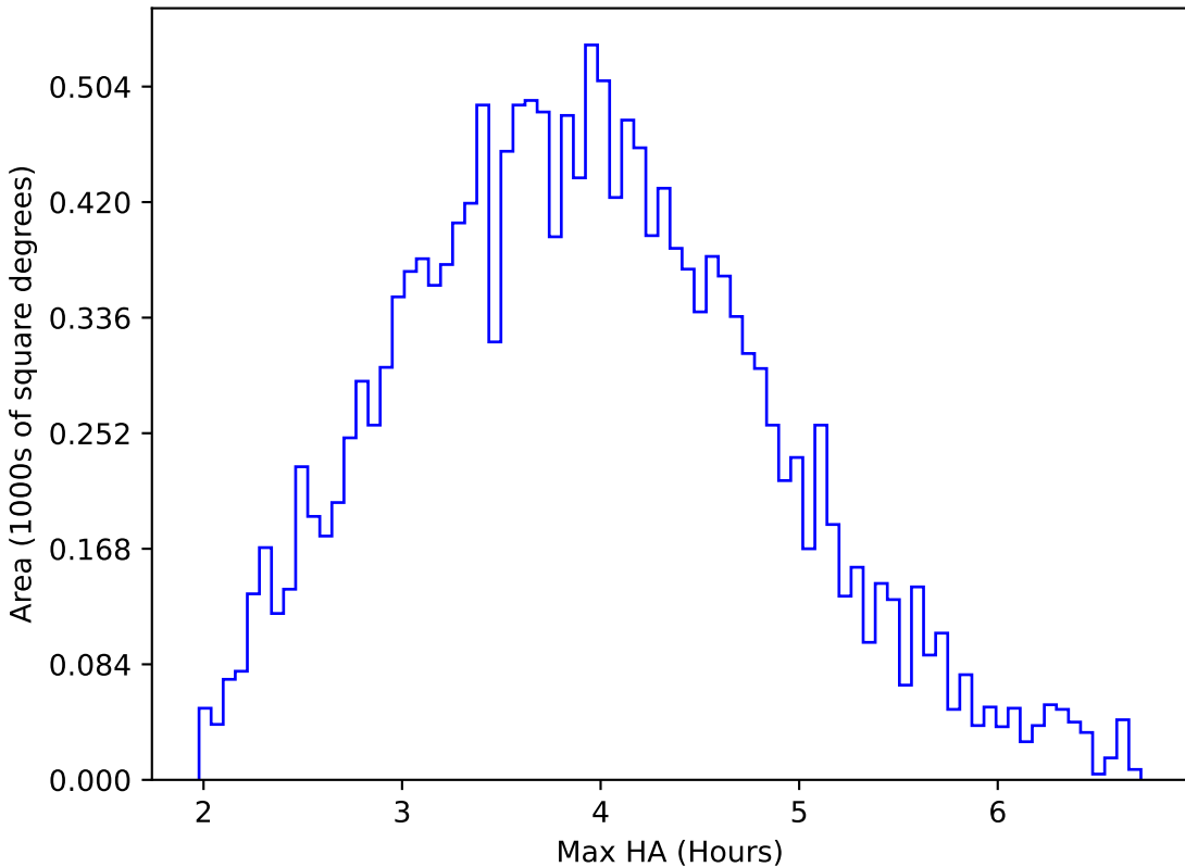
ddf_acor_sf10_lsf20_lsr20_v3.4_10yrs WFD u band: Max HA
