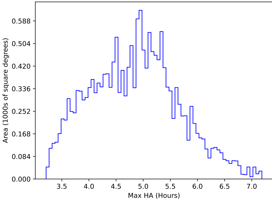
ddf_acor_sf10_lsf20_lsr20_v3.4_10yrs WFD i band: Max HA
