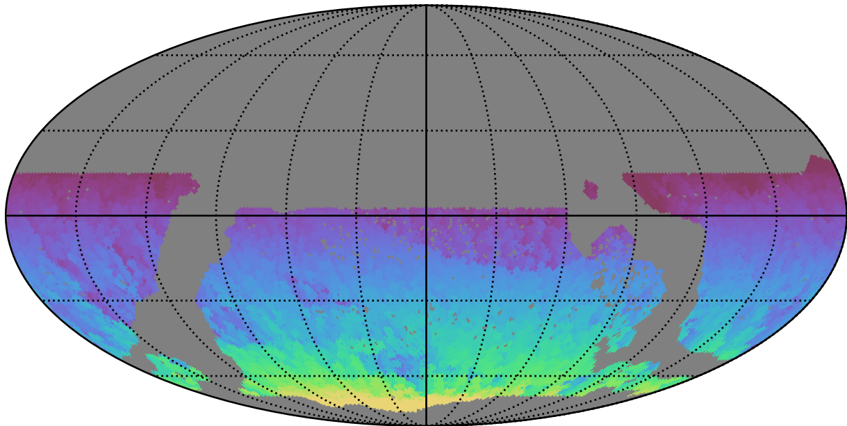
ddf_acor_sf10_lsf20_lsr20_v3.4_10yrs WFD all bands: Max HA
