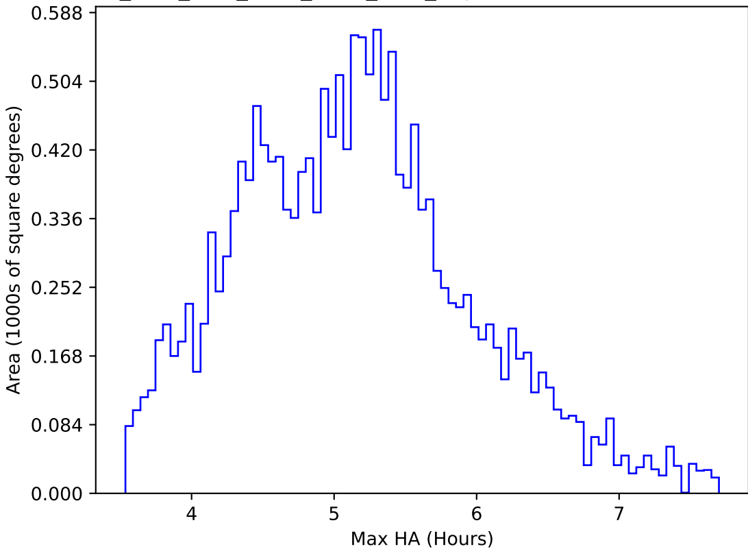
ddf_acor_sf10_lsf20_lsr20_v3.4_10yrs WFD all bands: Max HA
