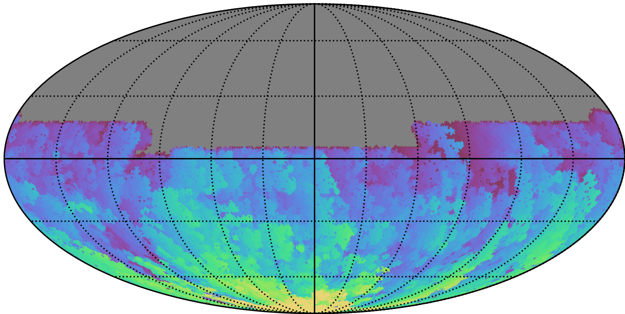
ddf_acor_sf10_lsf20_lsr20_v3.4_10yrs All sky u band: Max HA
