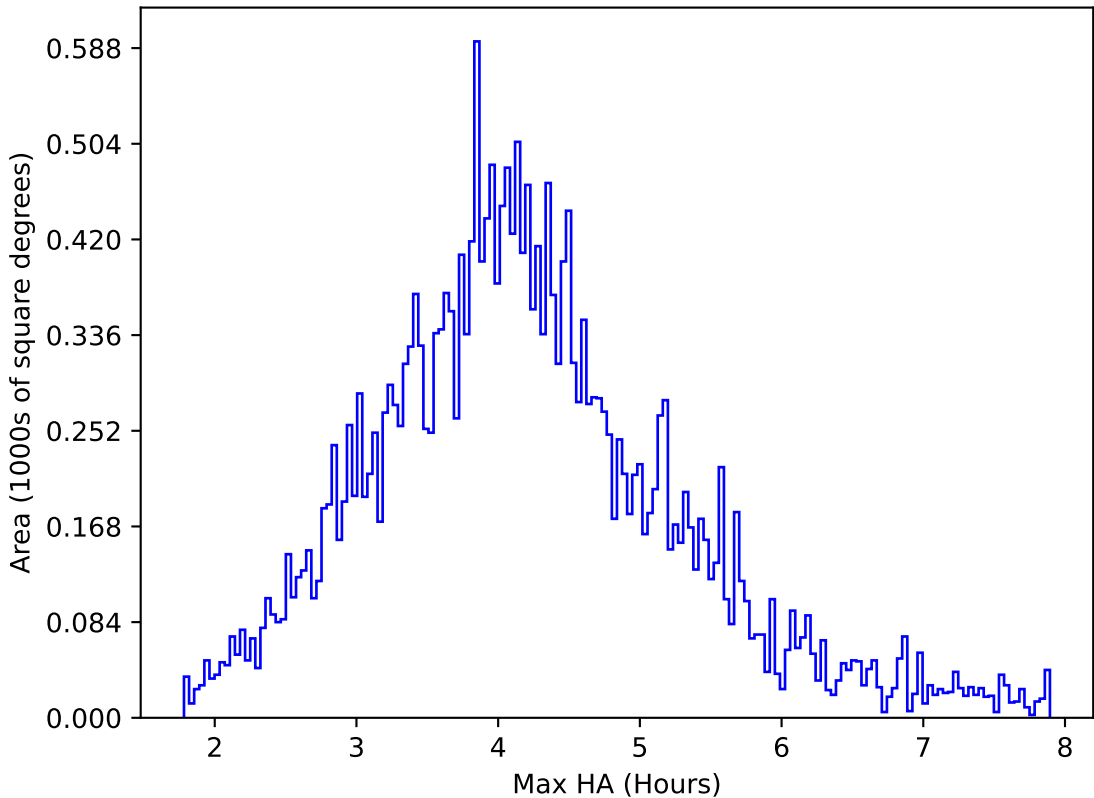
ddf_acor_sf10_ls20_lsr20_v3.4_10yrs All sky r band: Max HA
