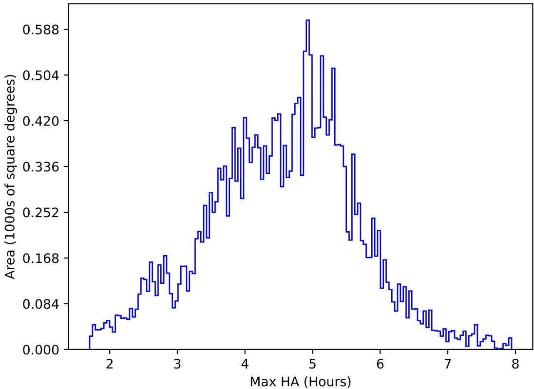
ddf_acor_sf10_lsf20_lsr20_v3.4_10yrs All sky i band: Max HA
