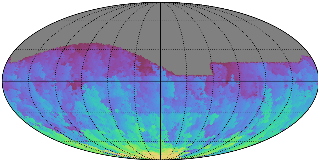
ddf_acor_sf10_lsf20_lsr20_v3.4_10yrs All sky g band: Max HA
