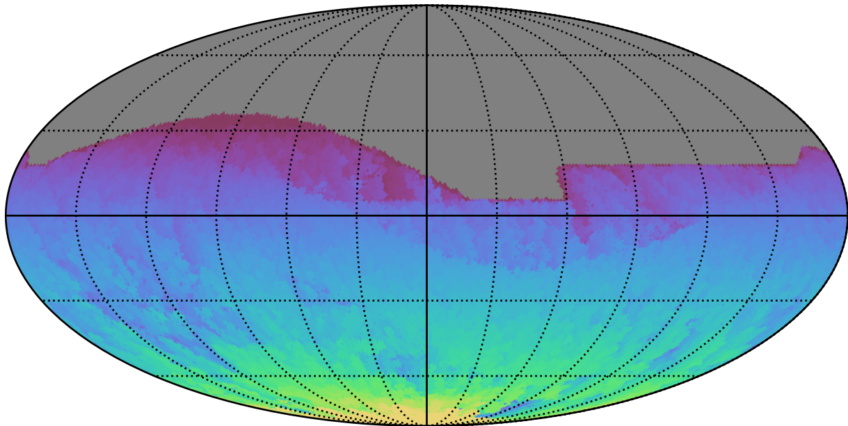
ddf_acor_sf10_lsf20_lsr20_v3.4_10yrs All sky all bands: Max HA
