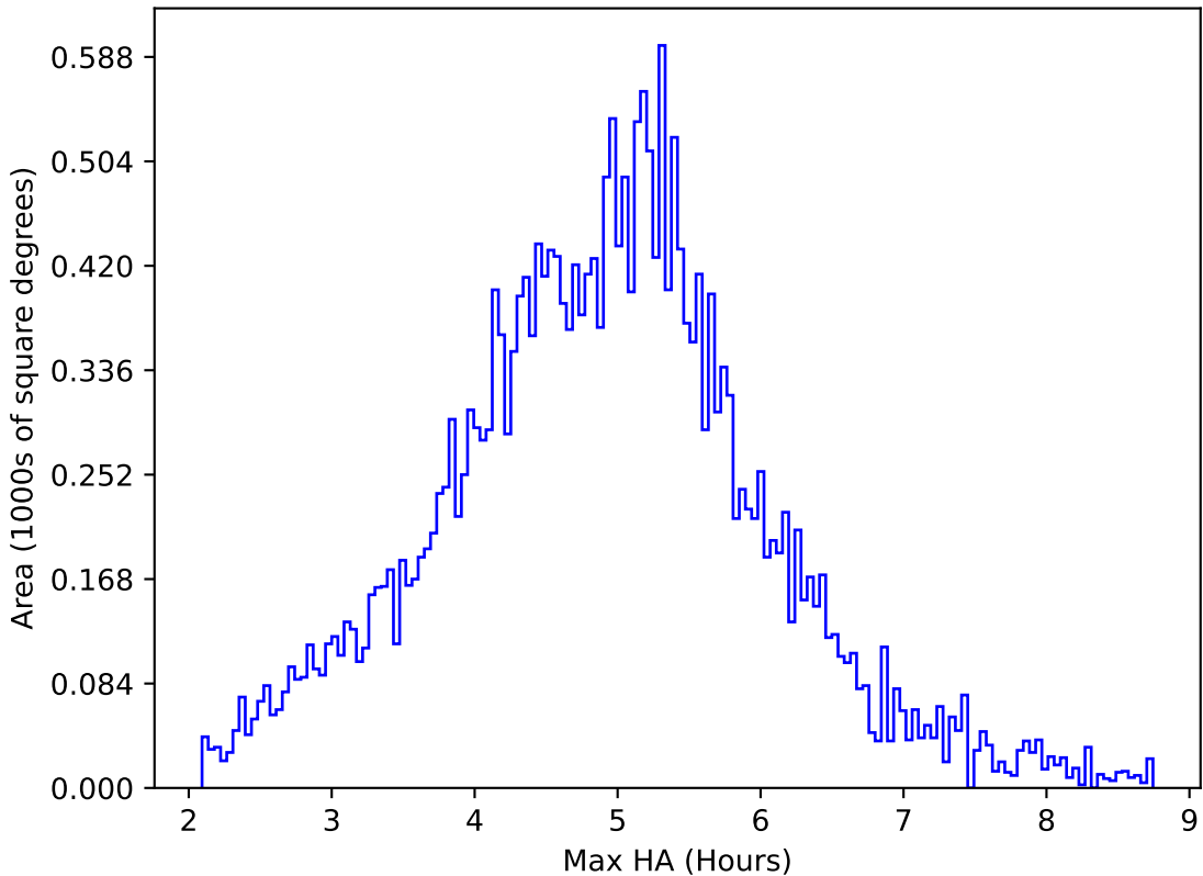
ddf_acor_sf10_lsf20_lsr20_v3.4_10yrs All sky all bands: Max HA
