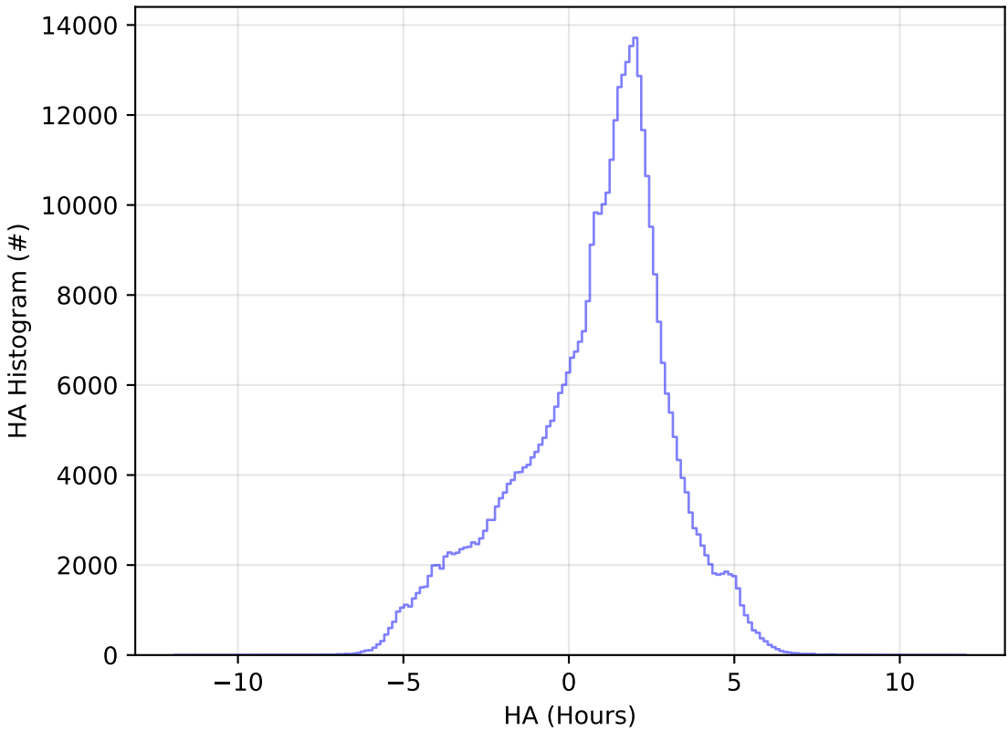
ddf_acor_sf10_lsf20_lsr20_v3.4_10yrs WFD z band: HA Histogram
