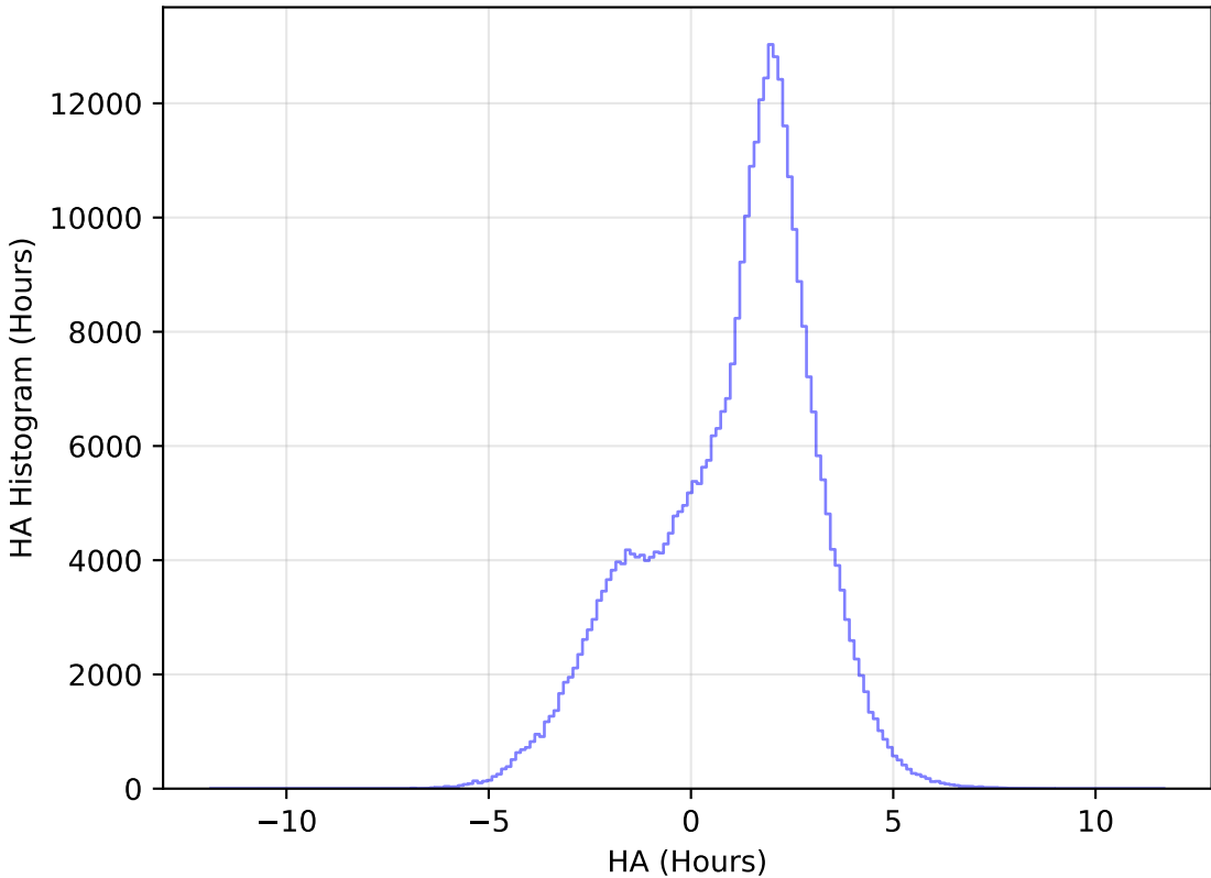
ddf_acor_sf10_lsf20_lsr20_v3.4_10yrs WFD y band: HA Histogram
