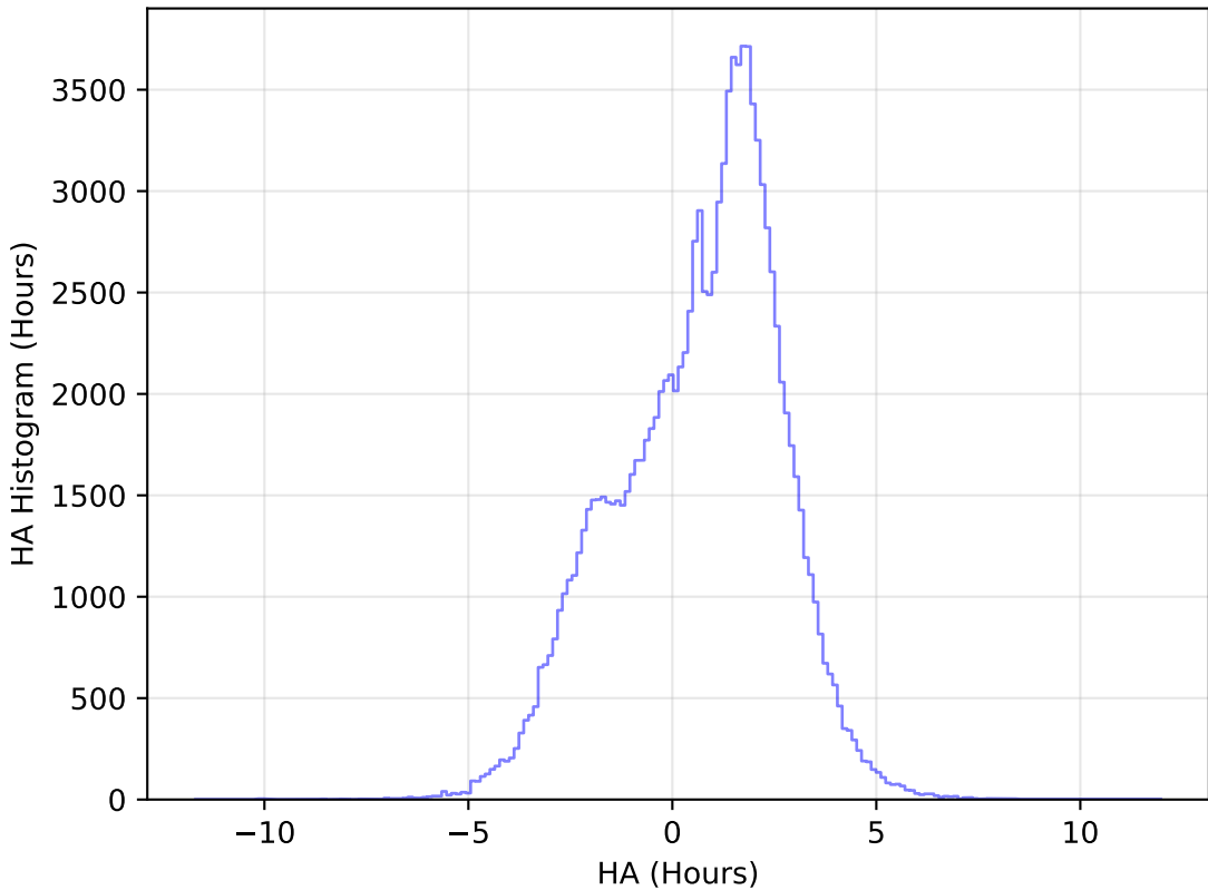
ddf_acor_sf10_lsf20_lsr20_v3.4_10yrs WFD u band: HA Histogram
