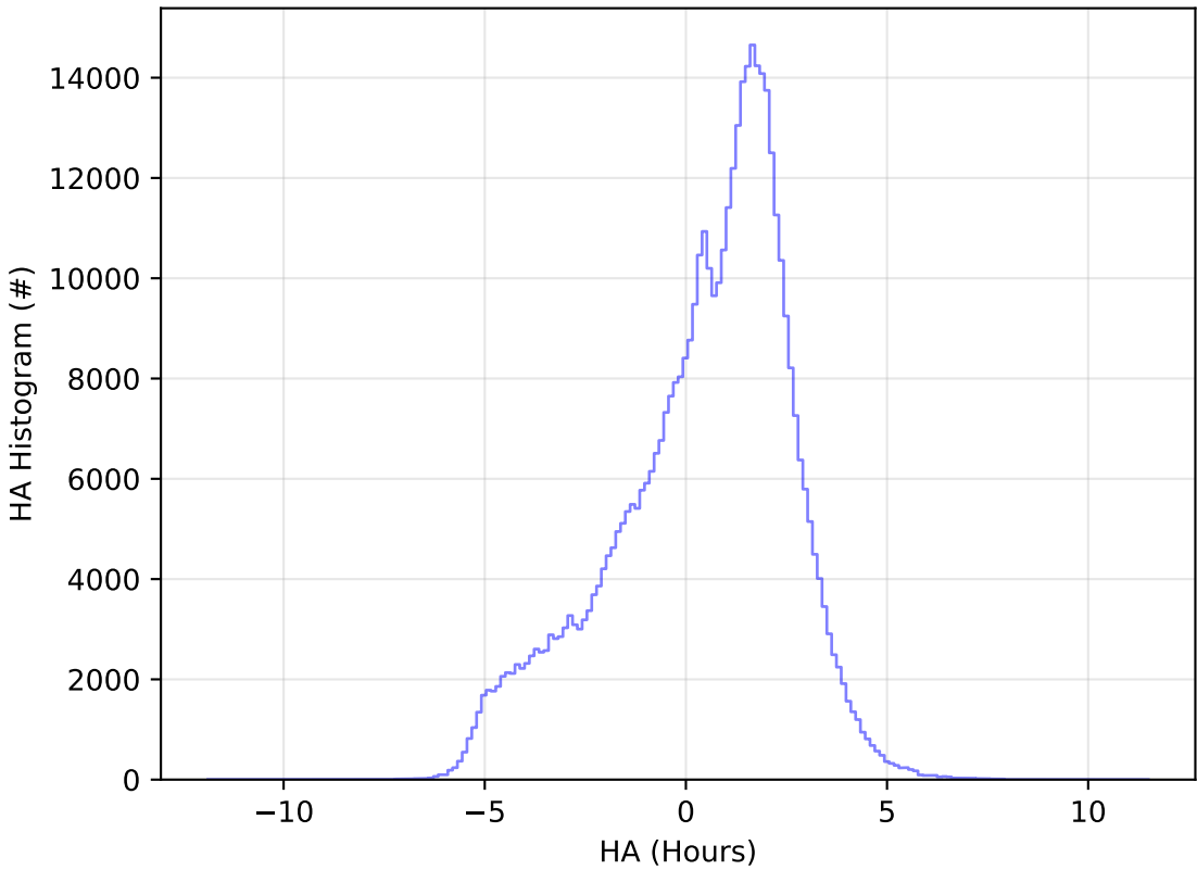
ddf_acor_sf10_lsf20_lsr20_v3.4_10yrs WFD r band: HA Histogram
