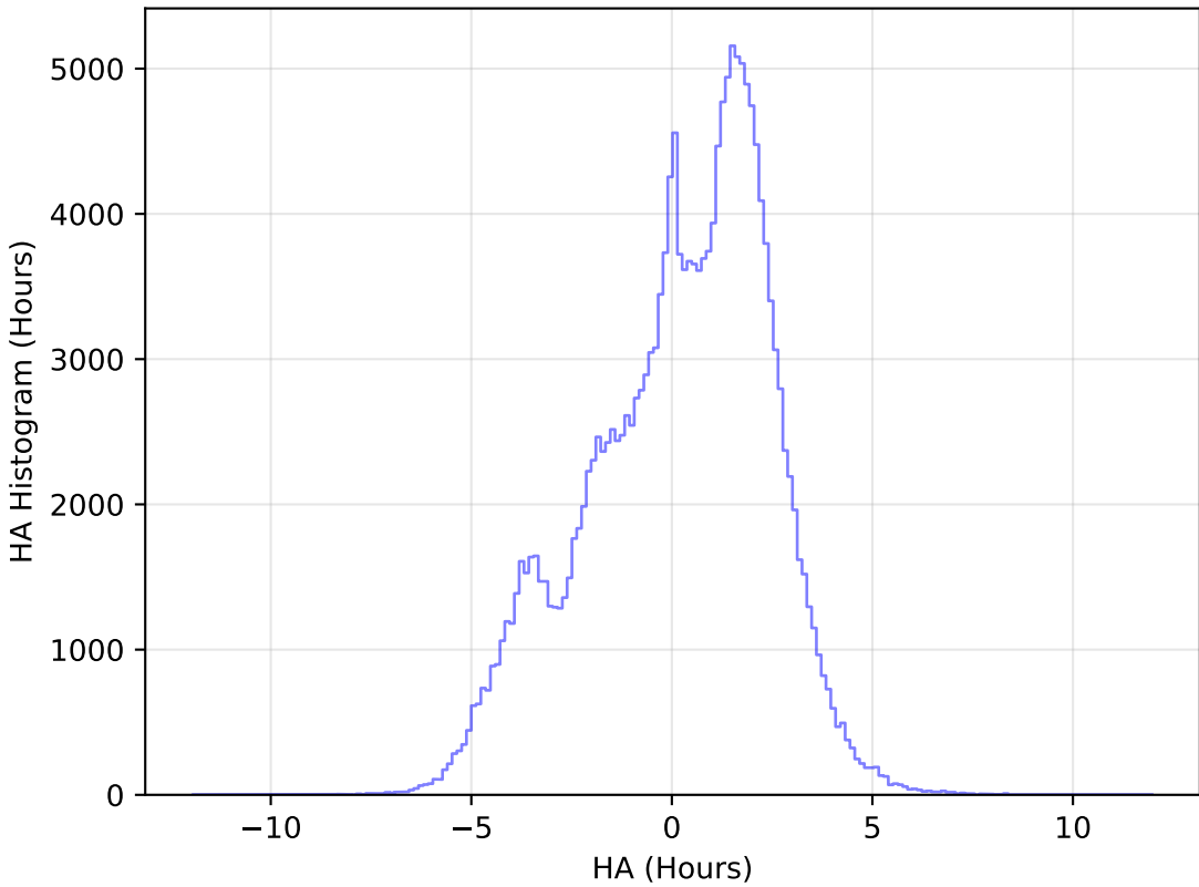
ddf_acor_sf10_lsf20_lsr20_v3.4_10yrs WFD g band: HA Histogram
