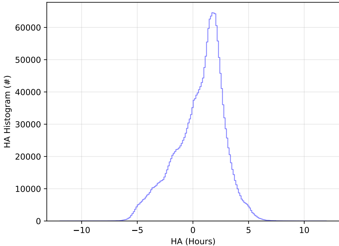
ddf_acor_sf10_lsf20_lsr20_v3.4_10yrs WFD all bands: HA Histogram
