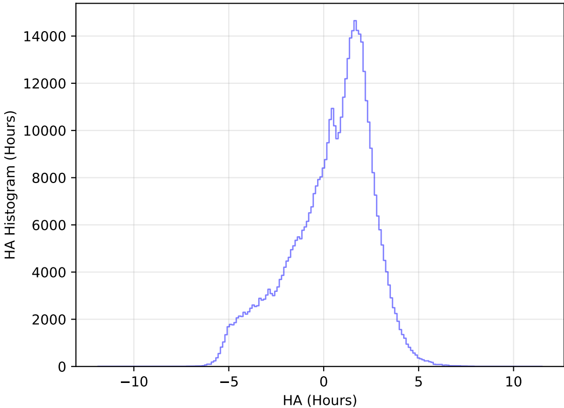
ddf_acor_sf10_lsf20_lsr20_v3.4_10yrs All sky r band: HA Histogram
