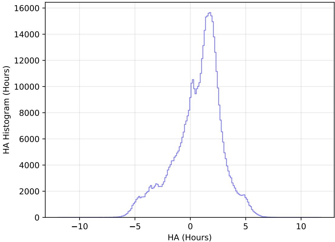
ddf_acor_sf10_lsf20_lsr20_v3.4_10yrs All sky i band: HA Histogram
