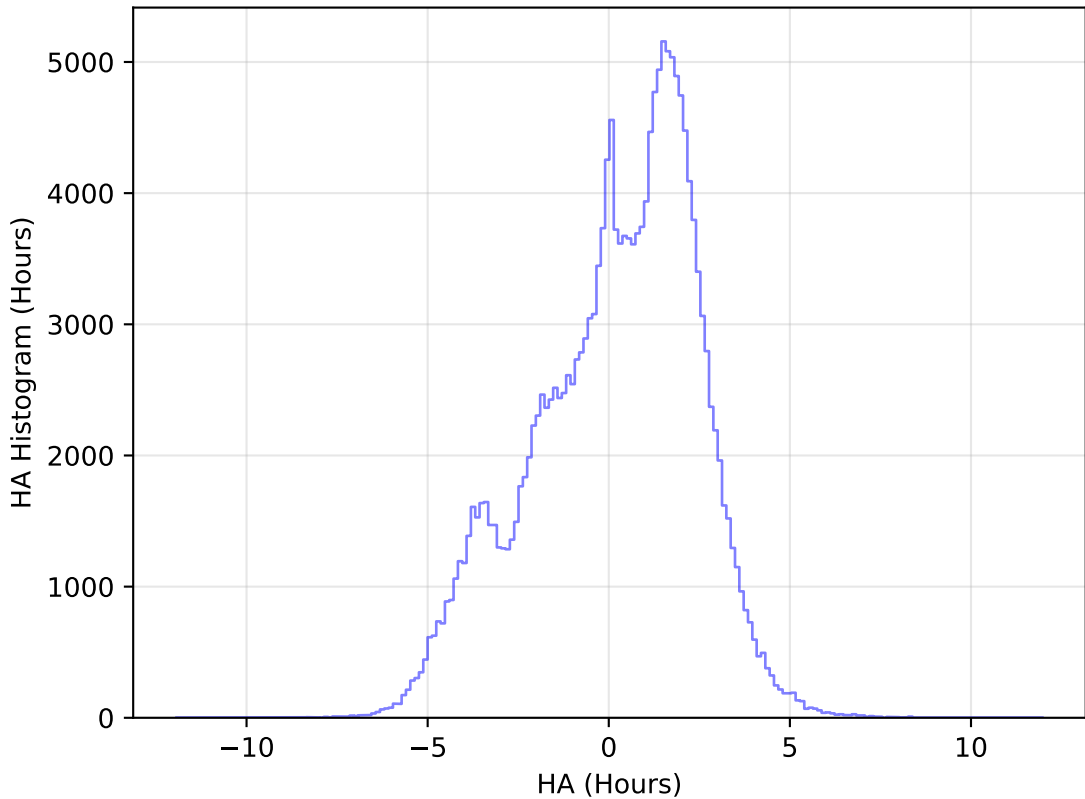
ddf_acor_sf10_lsf20_lsr20_v3.4_10yrs All sky g band: HA Histogram
