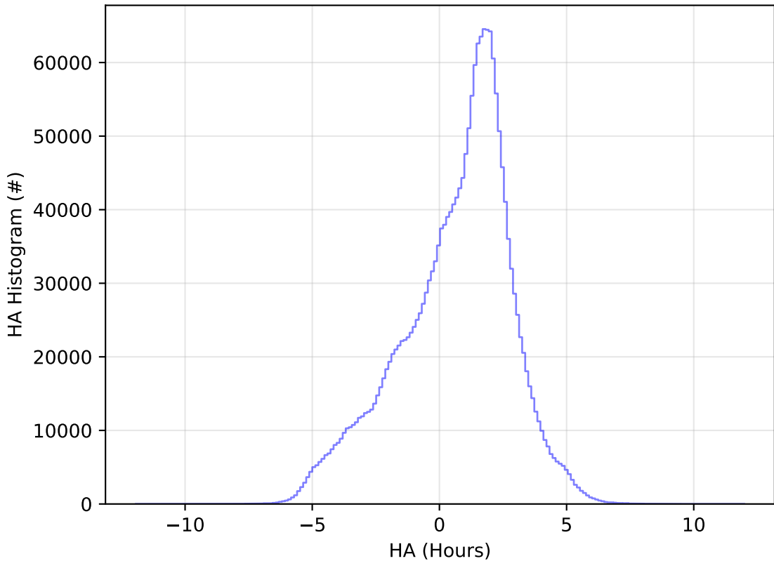
ddf_acor_sf10_lsf20_lsr20_v3.4_10yrs All sky all bands: HA Histogram
