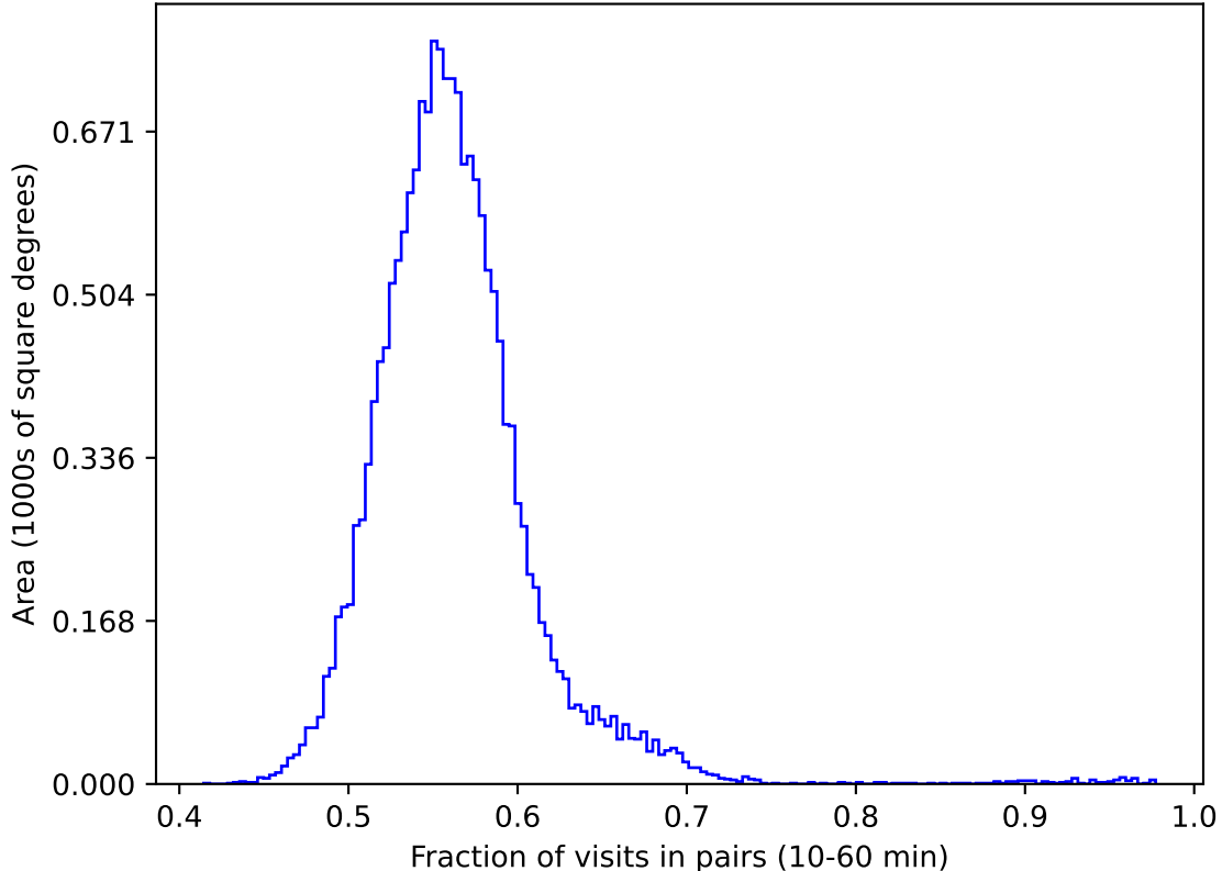
ddf_acor_sf10_lsf20_lsr20_v3.4_10yrs gri WFD: Fraction of visits in pairs (10-60 min)
