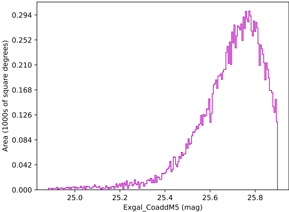
ddf_acor_sf10_lsf20_lsr20_v3.4_10yrs WFD z band: Exgal_CoaddM5
