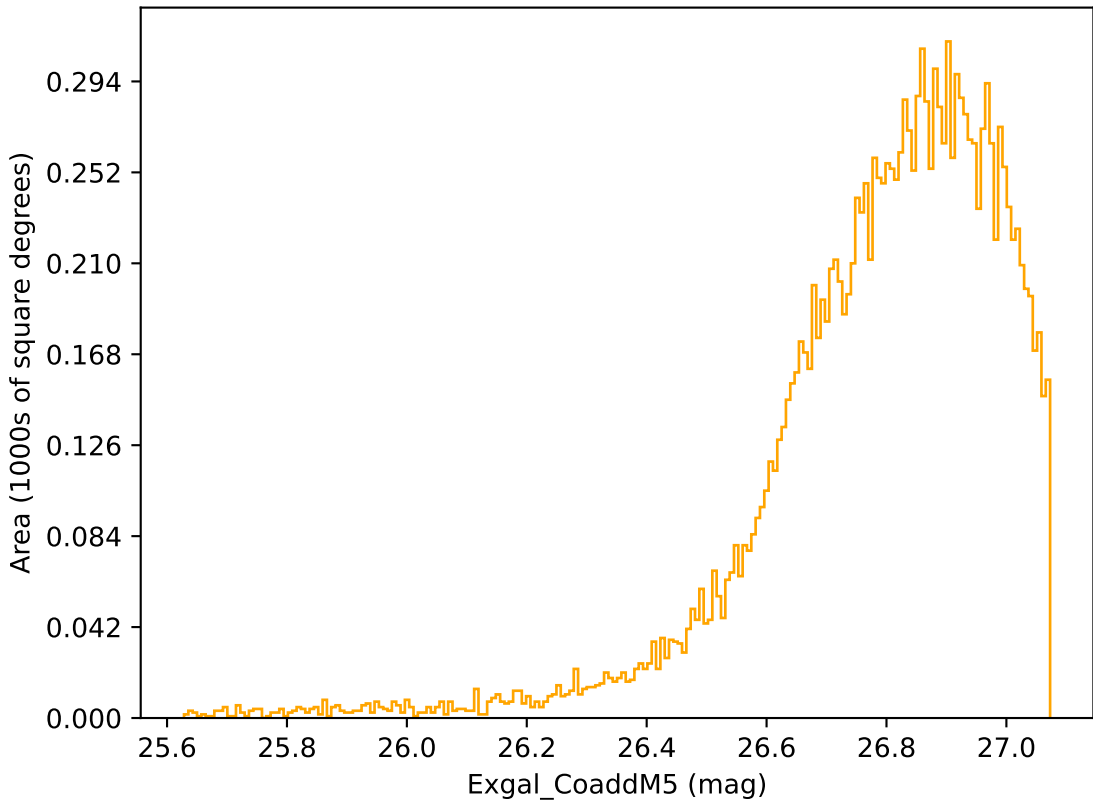
ddf_acor_sf10_lsf20_lsr20_v3.4_10yrs WFD r band: Exgal_CoaddM5
