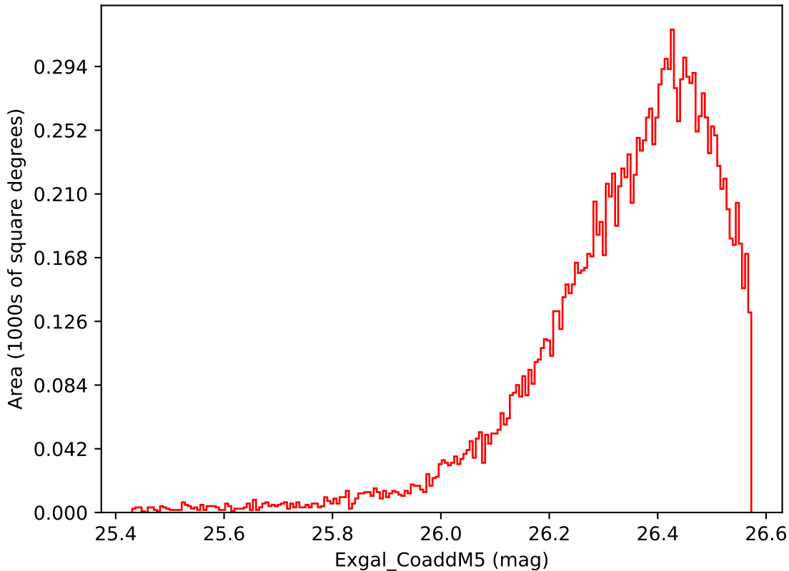
ddf_acor_sf10_lsf20_lsr20_v3.4_10yrs WFD i band: Exgal_CoaddM5
