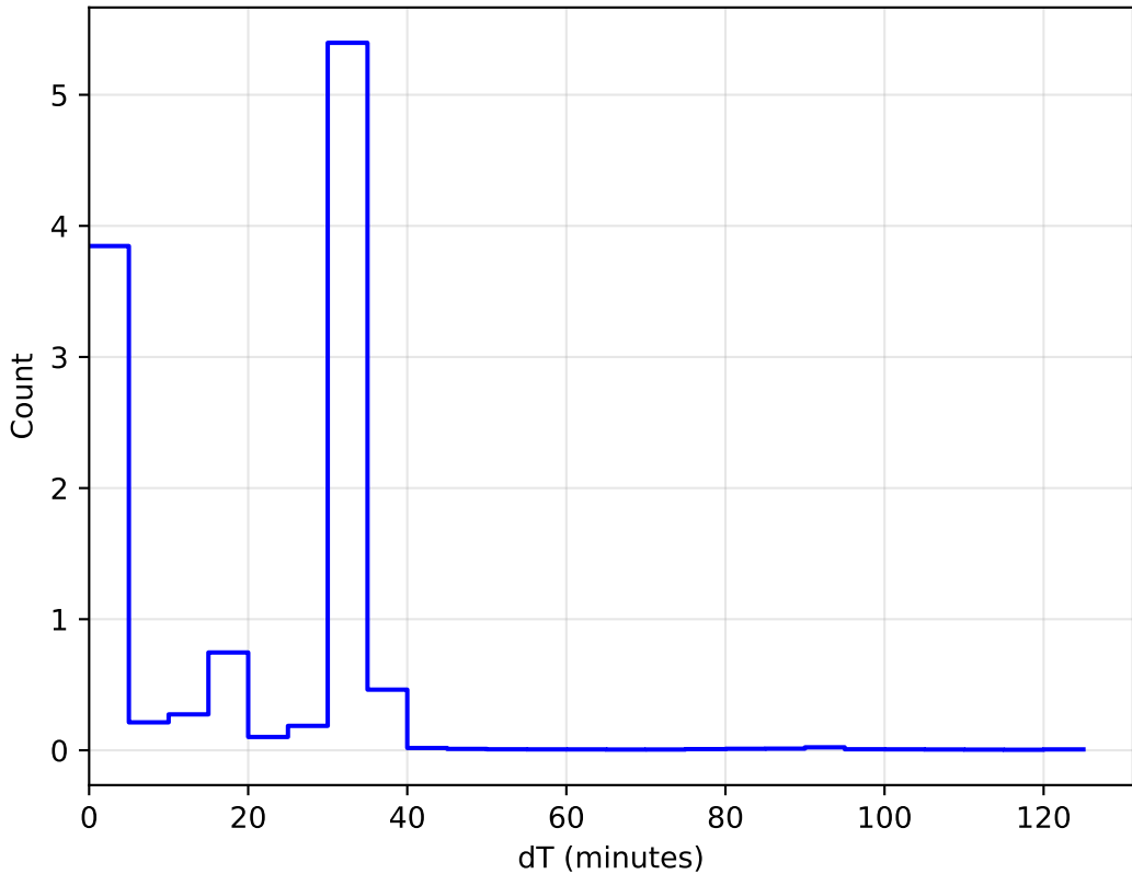
ddf_acor_sf10_lsf20_lsr20_v3.4_10yrs WFD: DeltaT Histogram 1e6
