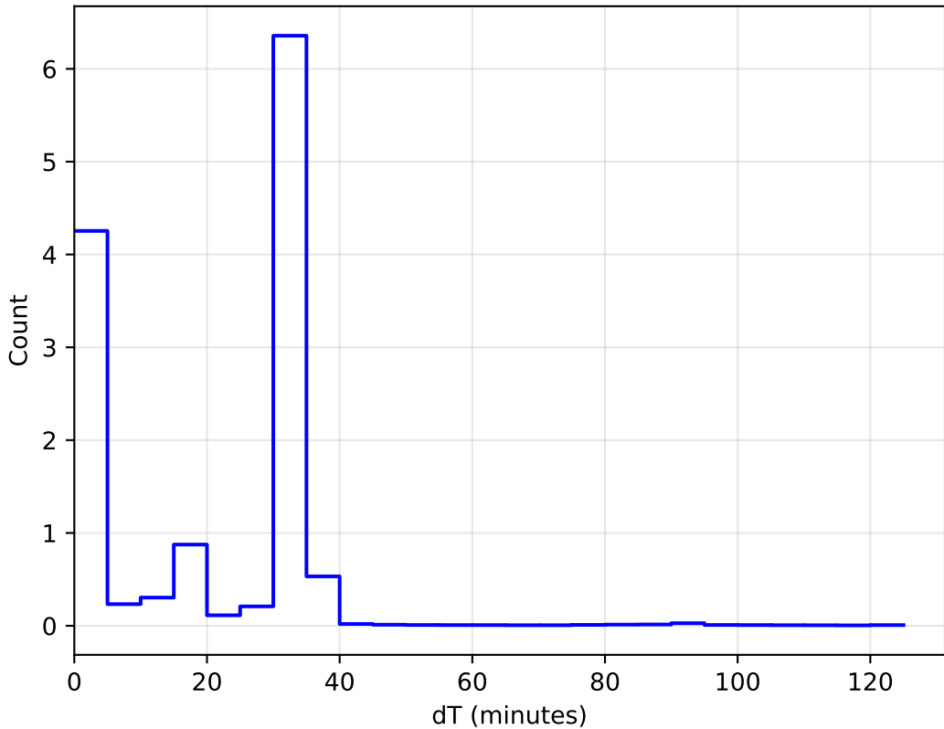
ddf_acor_sf10_lsf20_lsr20_v3.4_10yrs All sky: DeltaT Histogram
