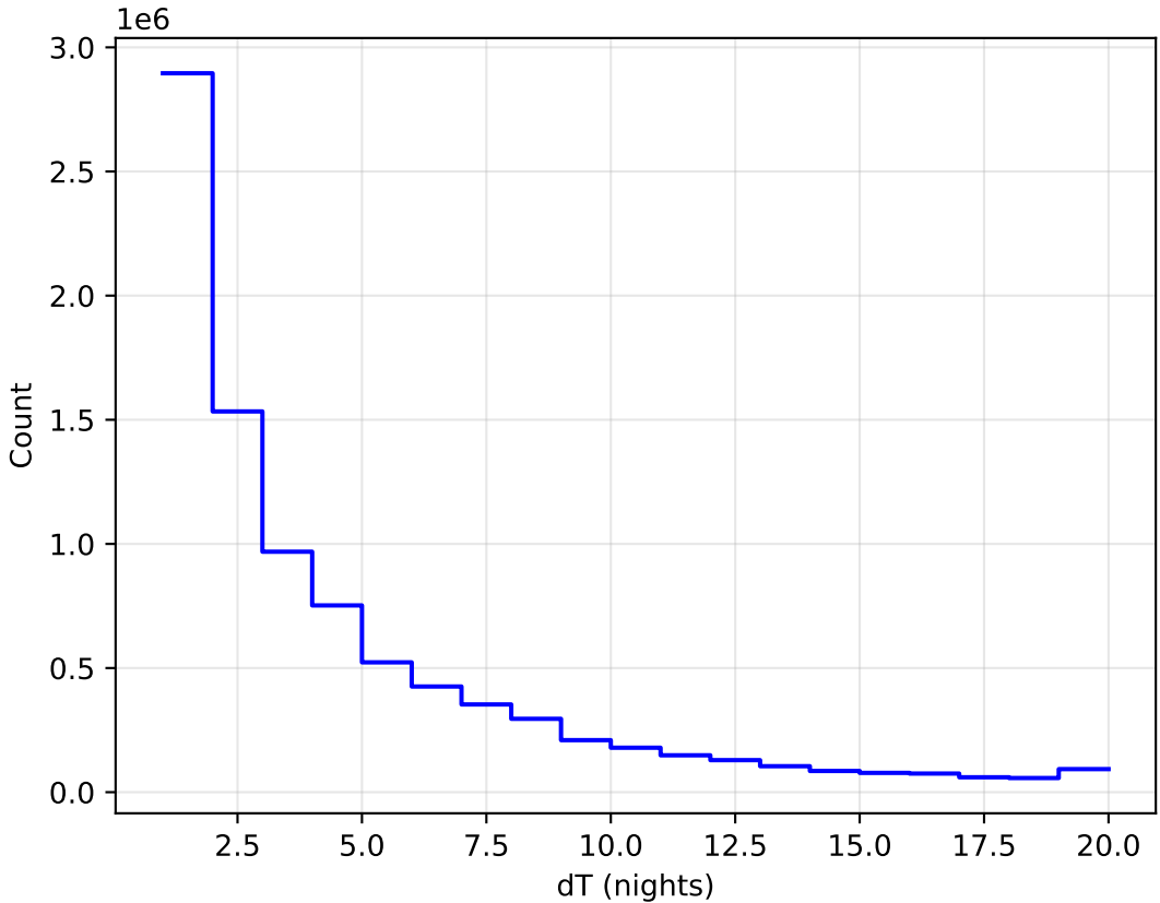
ddf_acor_sf10_lsf20_lsr20_v3.4_10yrs All sky all bands: DeltaNight Histogram
