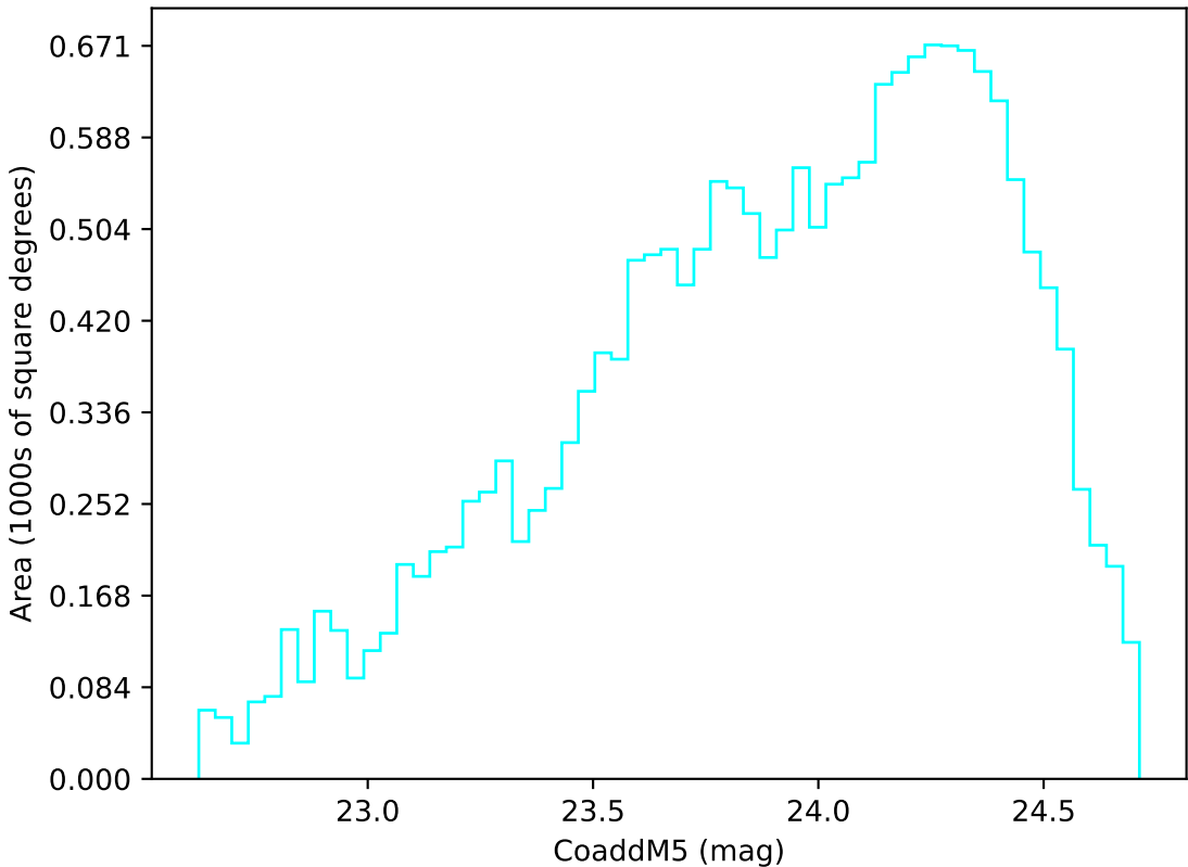
ddf_acor_sf10_lsf20_lsr20_v3.4_10yrs Yr 3-4 u band: CoaddM5
