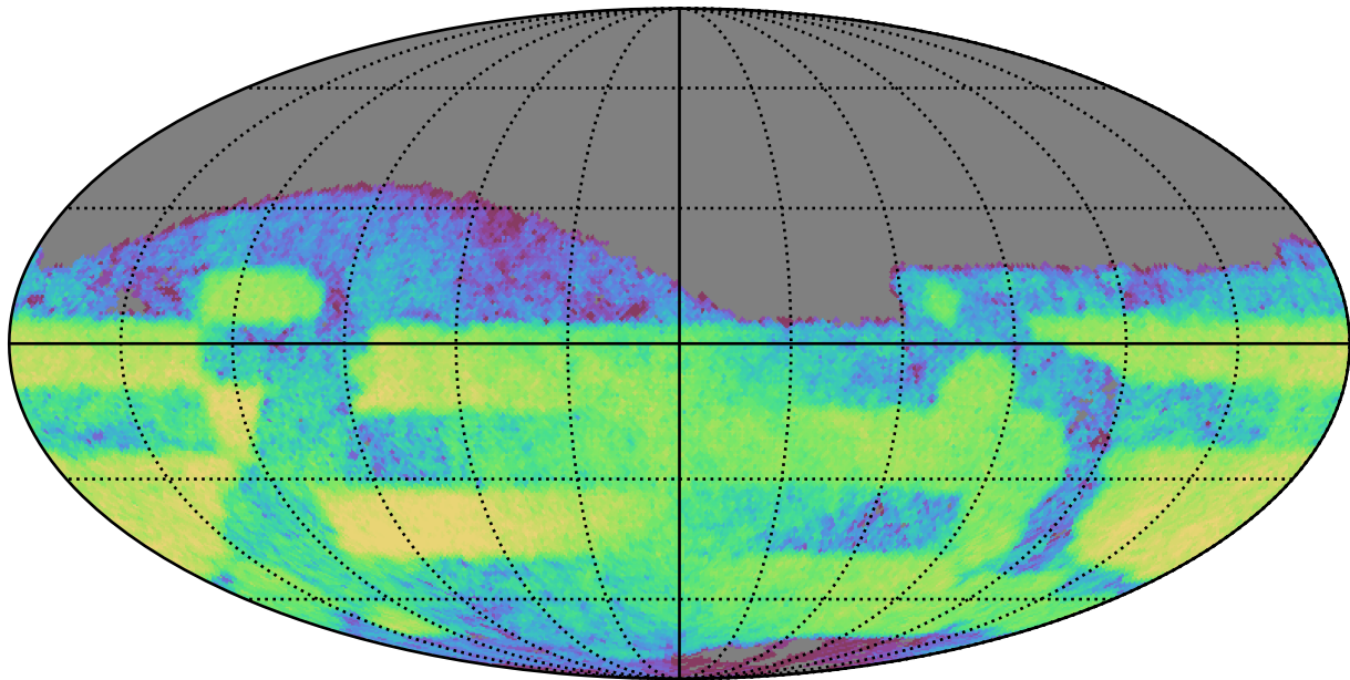
ddf_acor_sf10_lsf20_lsr20_v3.4_10yrs Yr 3-4 r band: CoaddM5
