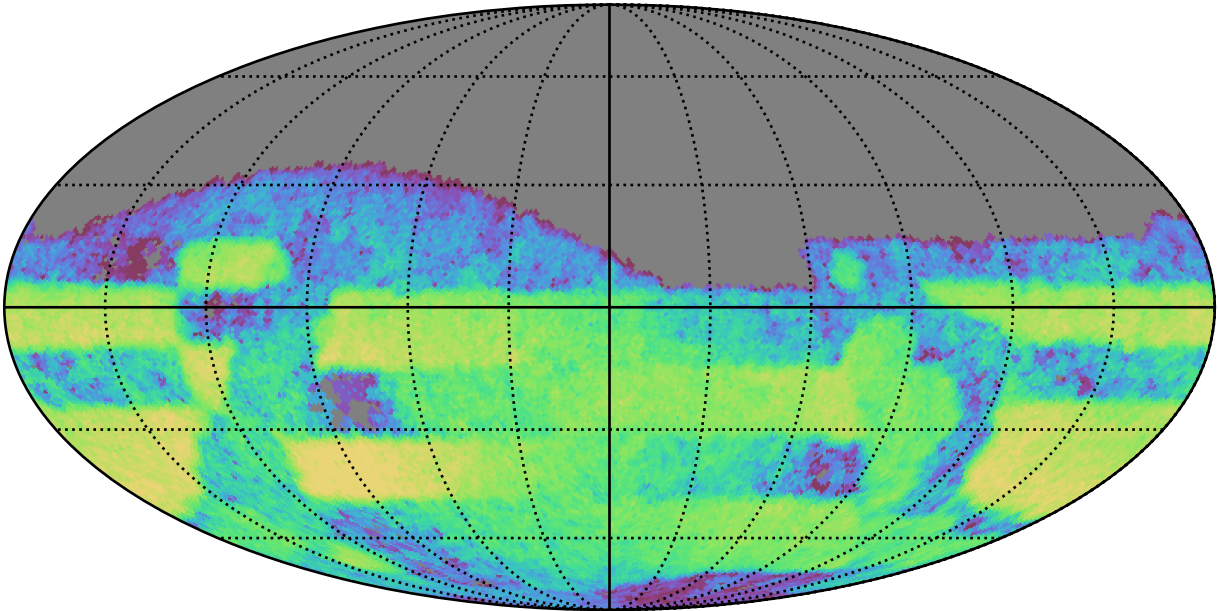
ddf_acor_sf10_lsf20_lsr20_v3.4_10yrs Yr 3-4 i band: CoaddM5
