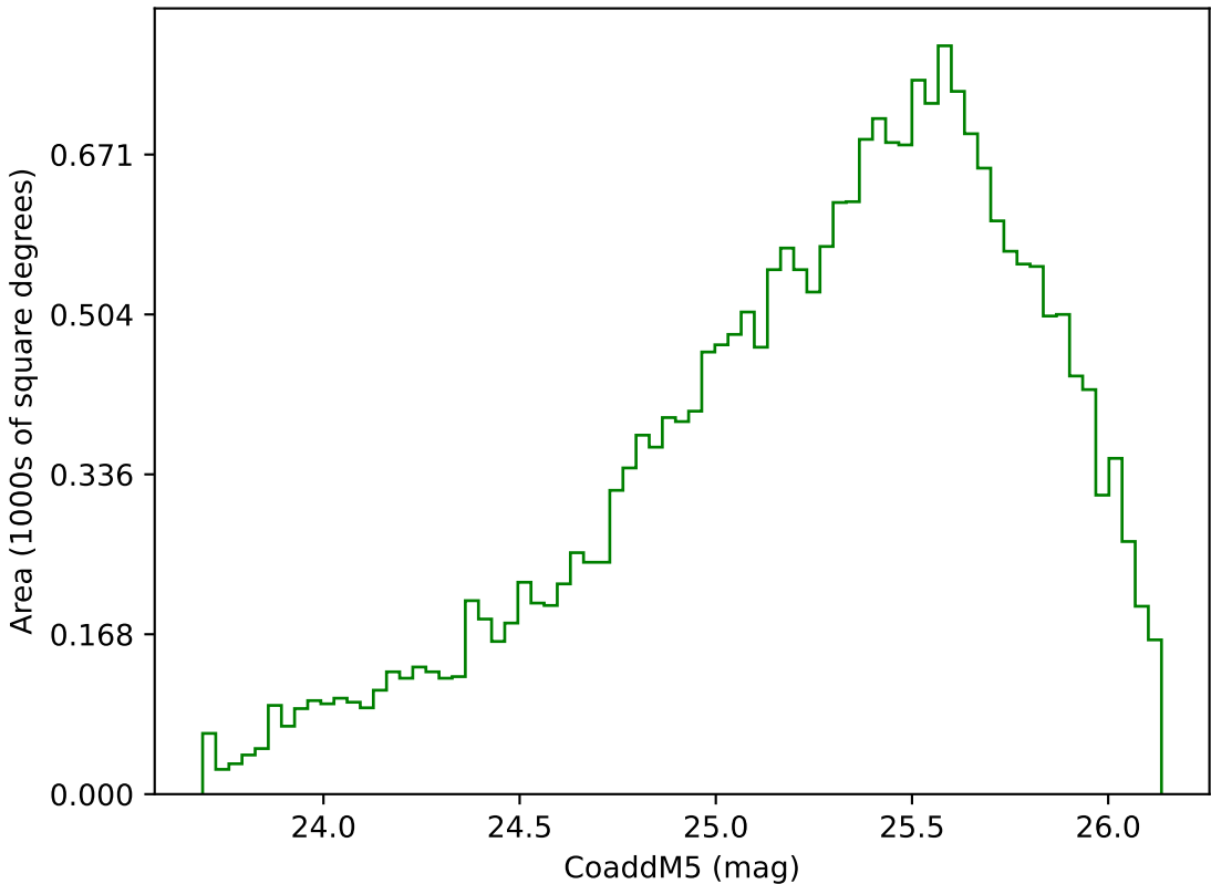
ddf_acor_sf10_lsf20_lsr20_v3.4_10yrs Yr 3-4 g band: CoaddM5
